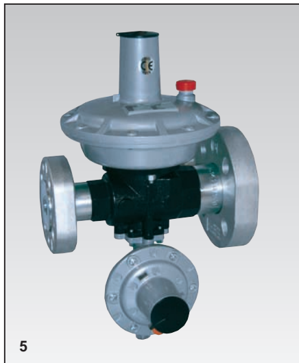
5 DIVAL 507 STANDARD CON BLOCCO E FLANGE SCORREVOLI DIVAL 507 STANDARD WITH SHUT-OFF DEVICE AND SLIDING FLANGES
